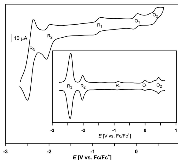
Figure 3. Cyclic and square-wave (inset) voltammograms of 6 in DMF containing 0.1 M TBAPFB, scan rate: 100 mV s −1 .
