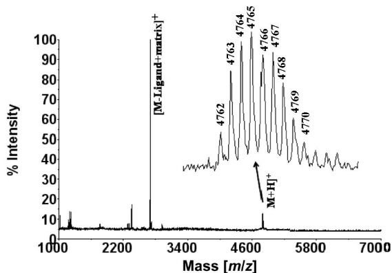
Figure 2. The positive-ion and reflectron mode MALDI-MS spectrum of 7 (lutetium) was obtained in dithranol (1,8-dihydroxy-10H-anthracen-9-one) (20 mg mL -1 tetrahydrofuran) MALDI matrix by using nitrogen laser accumulating 50 laser shots. Inset spectrum shows expanded molecular mass region of the complex.
