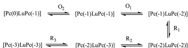
Scheme 2. The one-electron redox processes of Lu[(C 30 H 28 N 3 O) 4 ] 2 .
