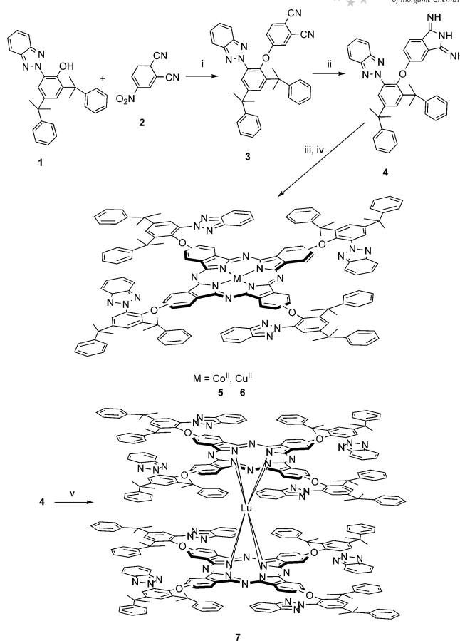
Scheme 1. (i) K 2 CO 3 , DMF, Ar; (ii) NH 3 , CH 3 ONa; (iii) Co(CH 3 COO) 2 ·4H 2 O, DMF, Ar; (iv) Cu(CH 3 COO) 2 ·2H 2 O, DMF, Ar; (v) Lu(CH 3 COO) 3 ·H 2 O, DBU, octanol, Ar.
