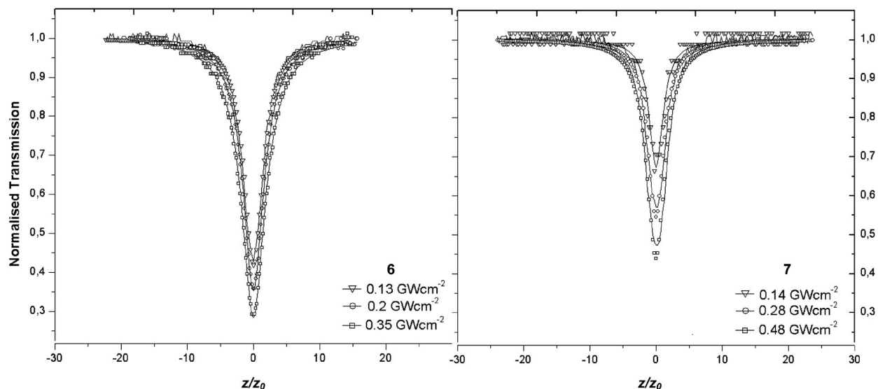
Figure 5. Normalized Z-scan experiment results for 6 and 7 under open-aperture configuration. Solid lines represent theoretical fits.
