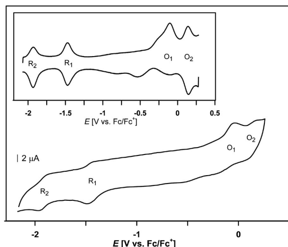
Figure 4. Cyclic and square-wave (inset) voltammograms of 7 in DMF containing 0.1 M TBAFB, scan rate: 100 mV s -1 .
