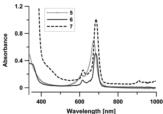
Figure 1. UV/Vis spectra of 5 , 6 , and 7 in THF.
