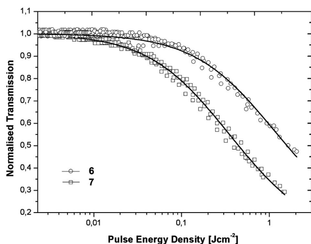
Figure 6. Plots of normalized transmission against incident pulse energy density for 6 and 7 . Solid lines represent theoretical fits.
